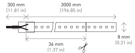
IP20 100W (168 LEDs/m)
