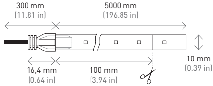
IP67 24W (60 LEDs/m)
