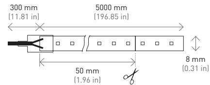
IP20 120W (120 LEDs/m)
