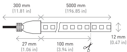
IP67 72W (60 LEDs/m)
