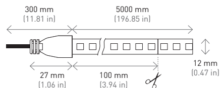
IP67 72W (60 LEDs/m)
